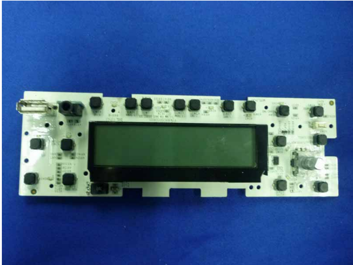
Figure 13 General Inside of the EUT
