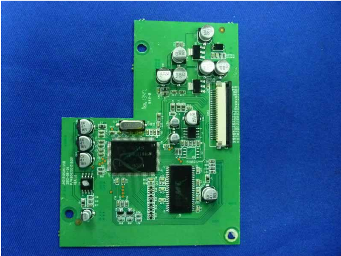
Figure 9 General Inside of the EUT
