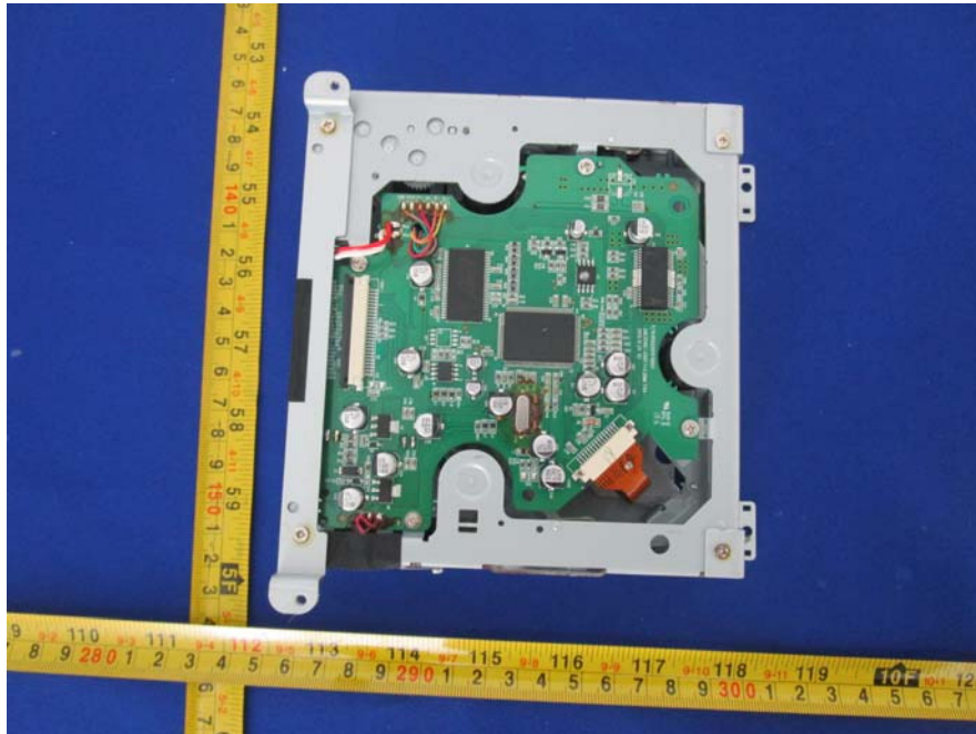
EUT – CD Bottom View
