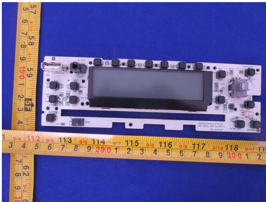
EUT –Panel Board Top View
