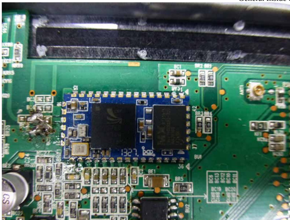
Figure 34 General Inside of the EUT
