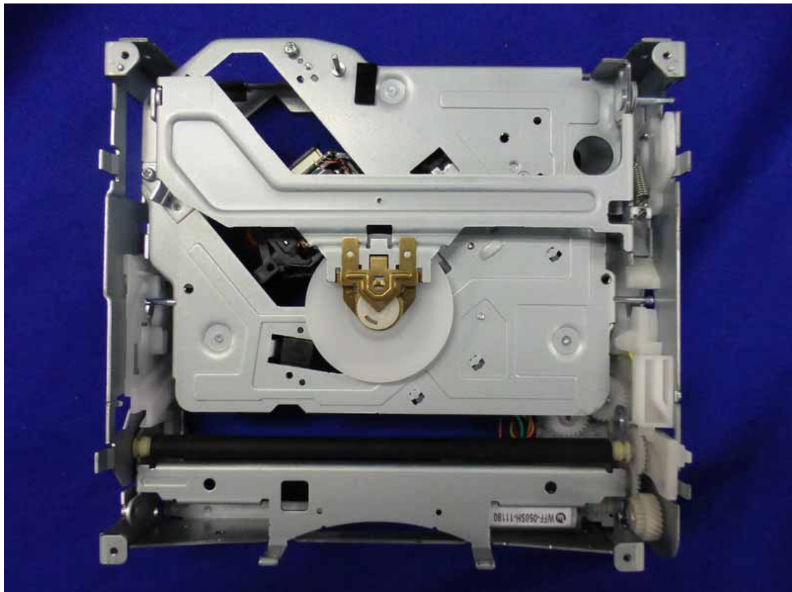
Figure 38 General Inside of the EUT
