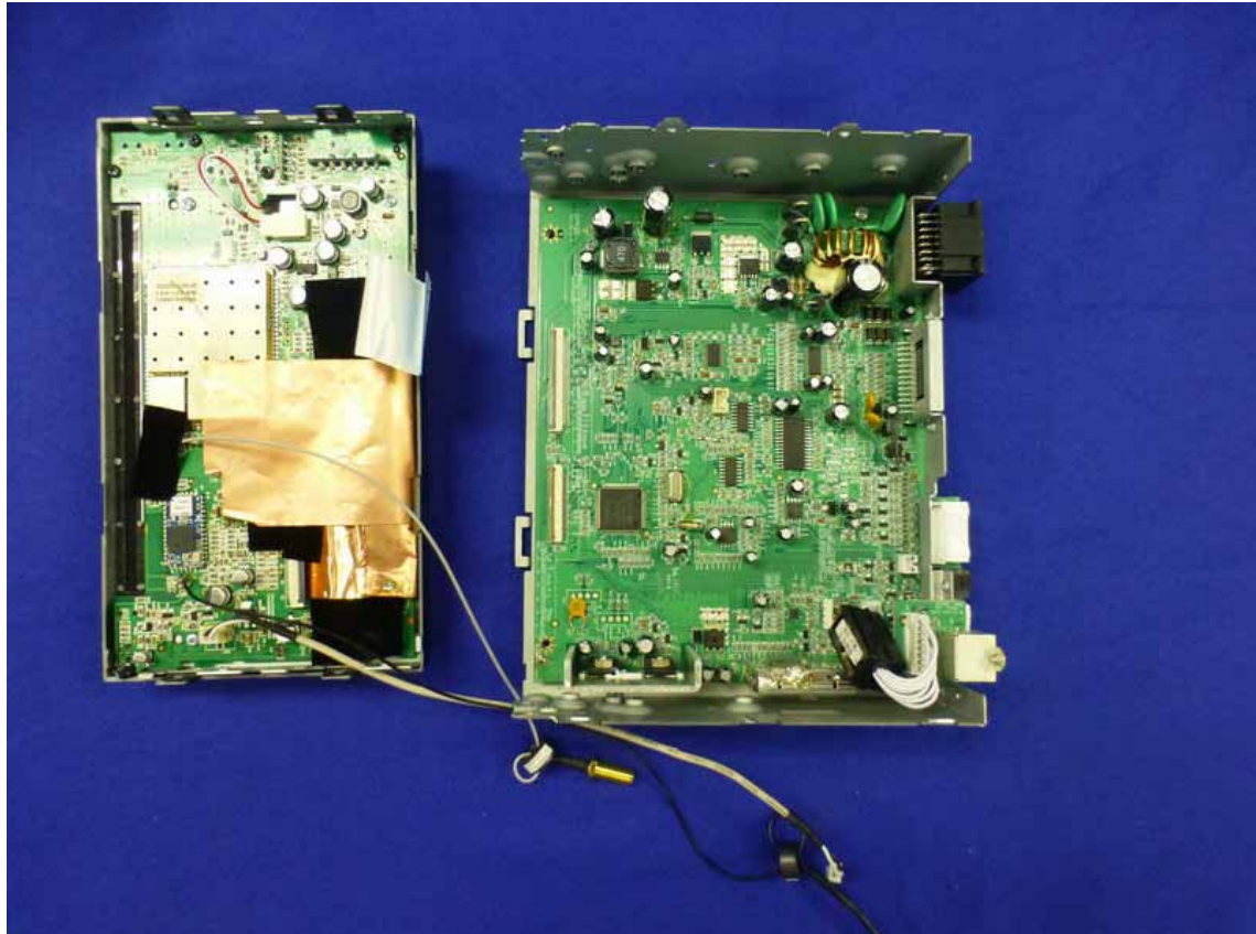
Figure 18 General Inside of the EUT
