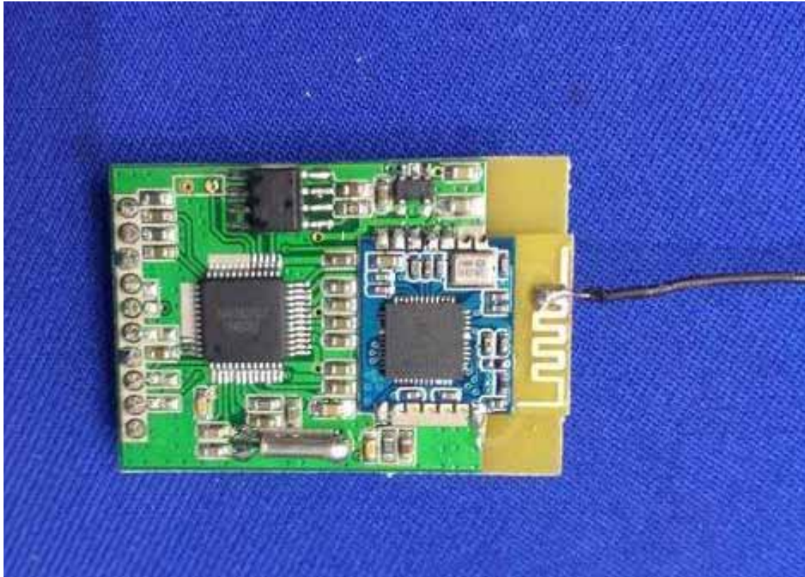
Figure 15 Inside of the EUT
