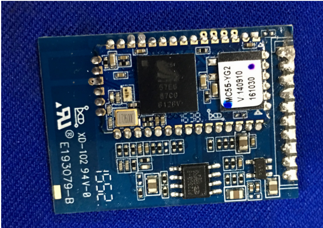
Figure 18 Inside of the EUT
