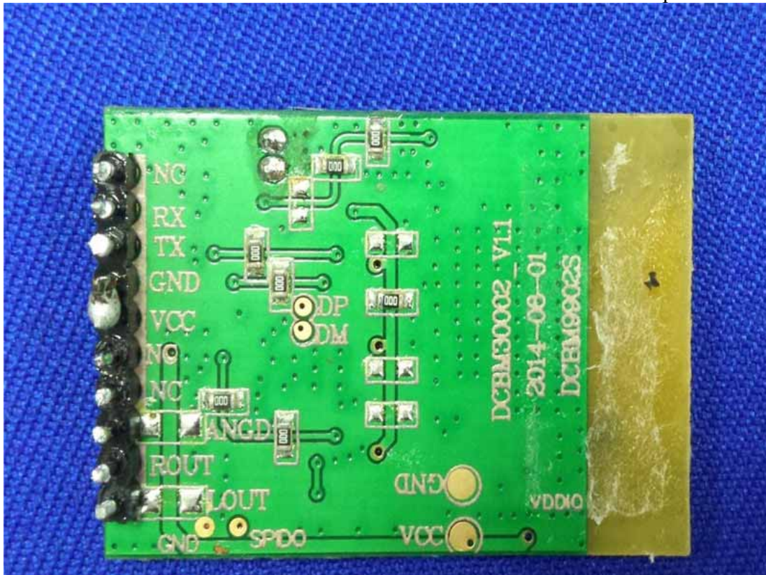
Figure 14 Component side of the PCB
