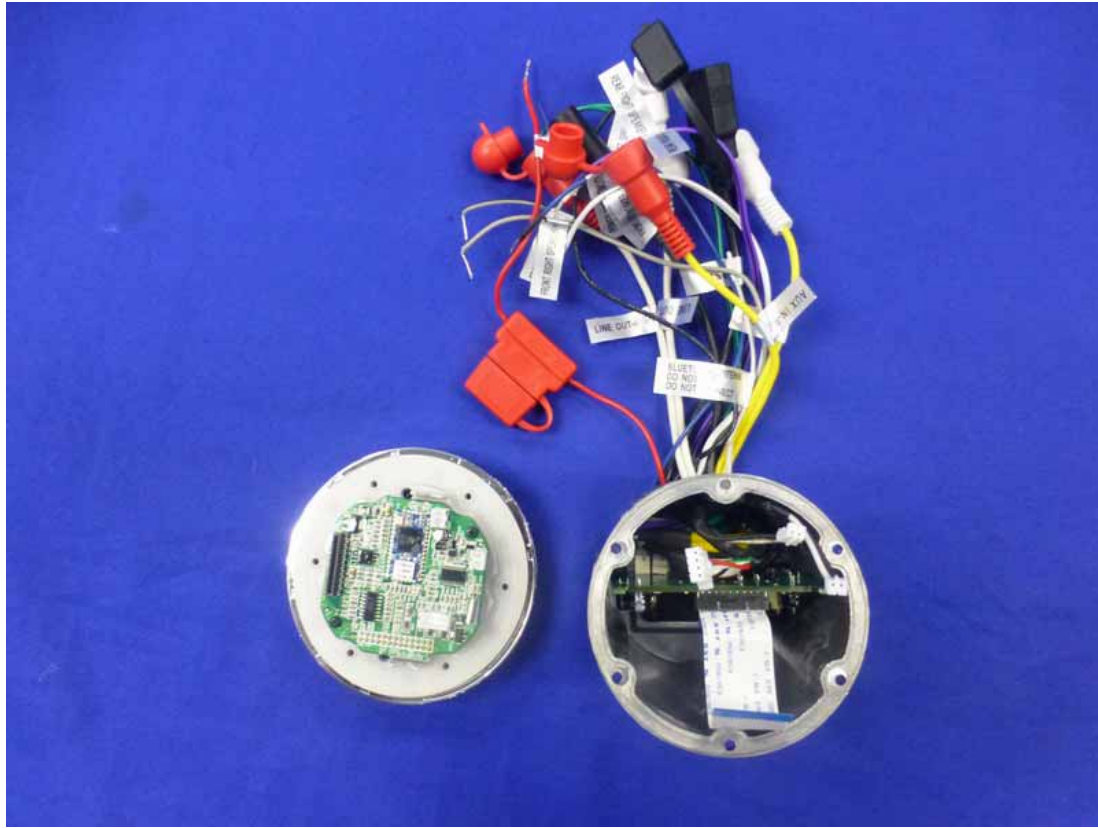
Figure 7 General Inside of the EUT
