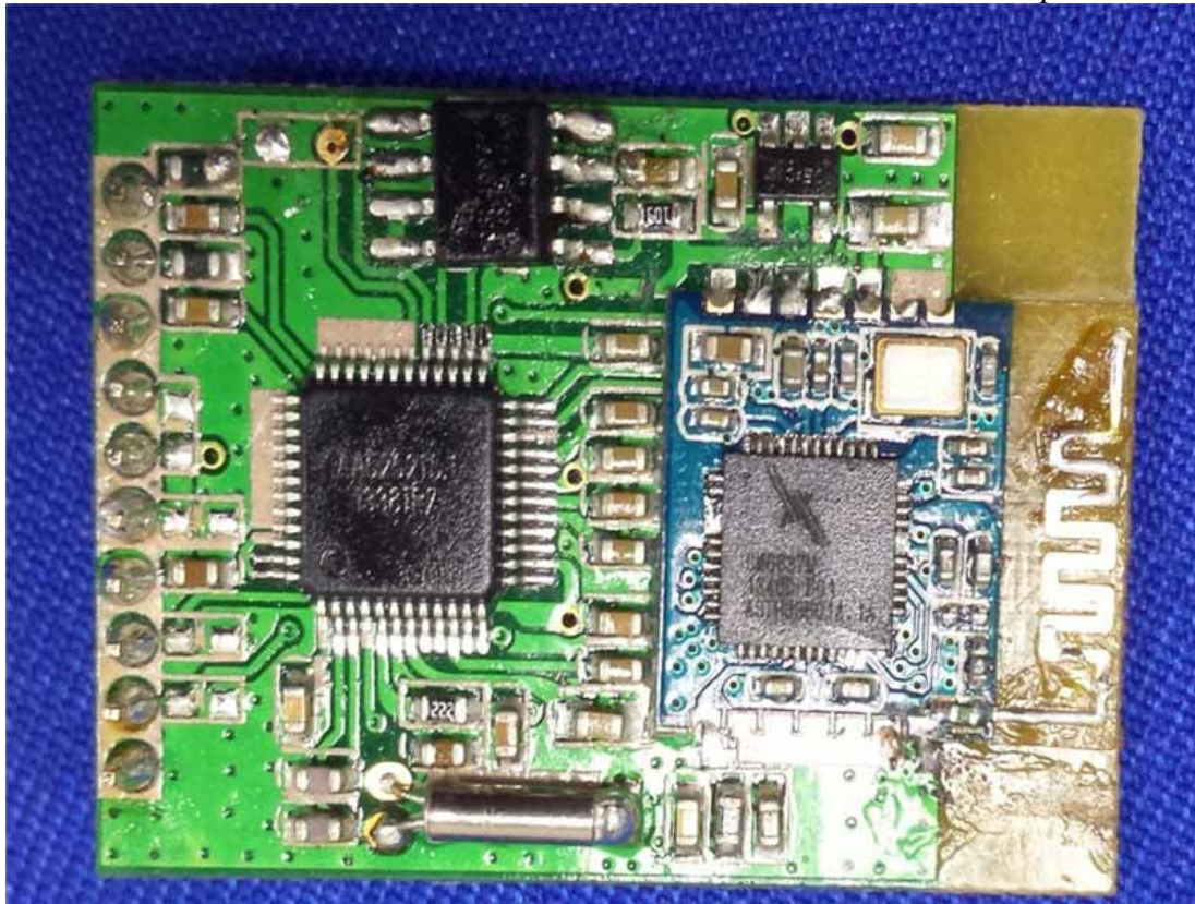
Figure 15 Component side of the PCB
