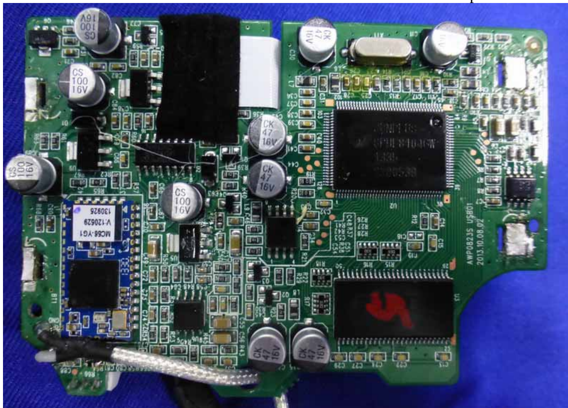
Figure 12 Component side of the PCB
