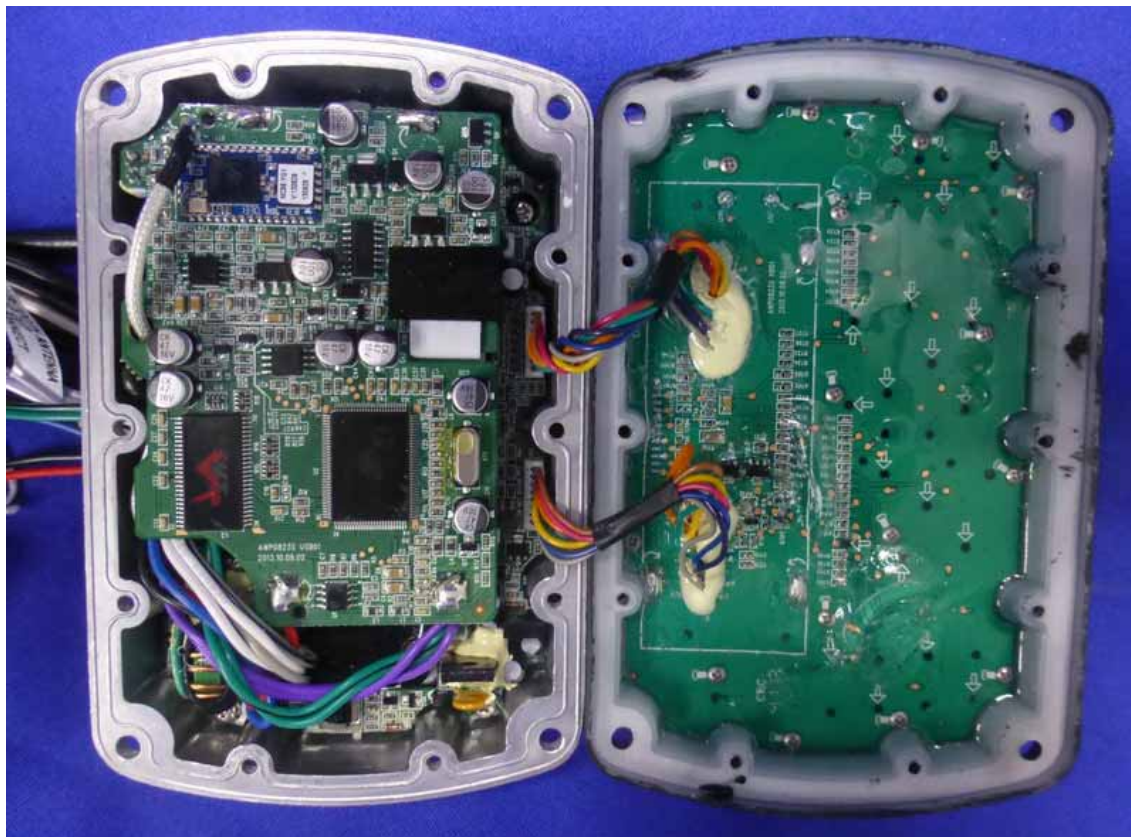
Figure 7 General Inside of the EUT
