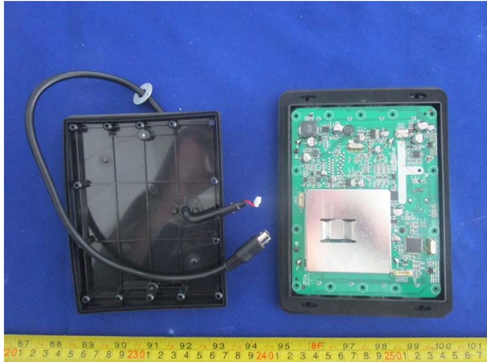
EUT – Controller Panel Uncover View
