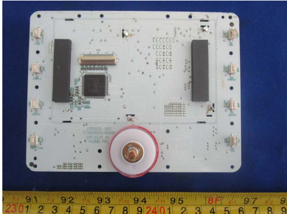
EUT – Controller Panel Mainboard Bottom Uncover View
