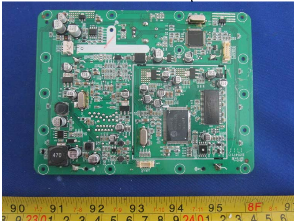
EUT – Controller Panel Mainboard Top Uncover View
