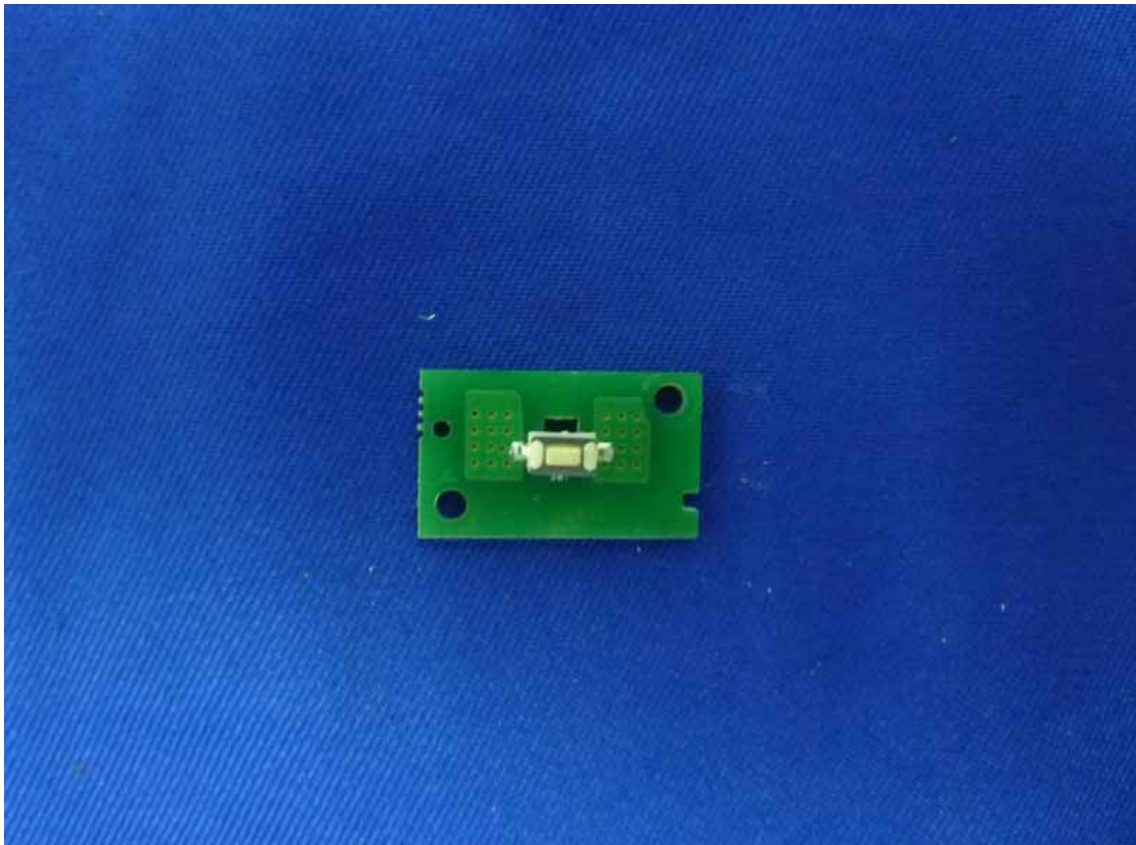
Figure 26 General Inside of the EUT
