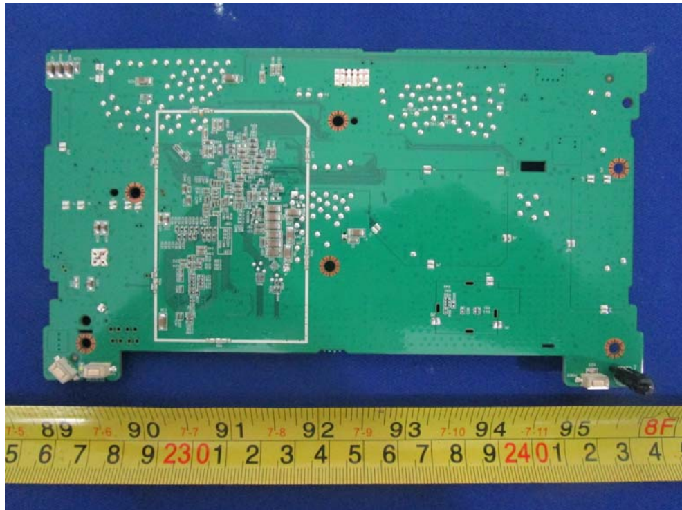
EUT – Subboard Bottom Uncover View
