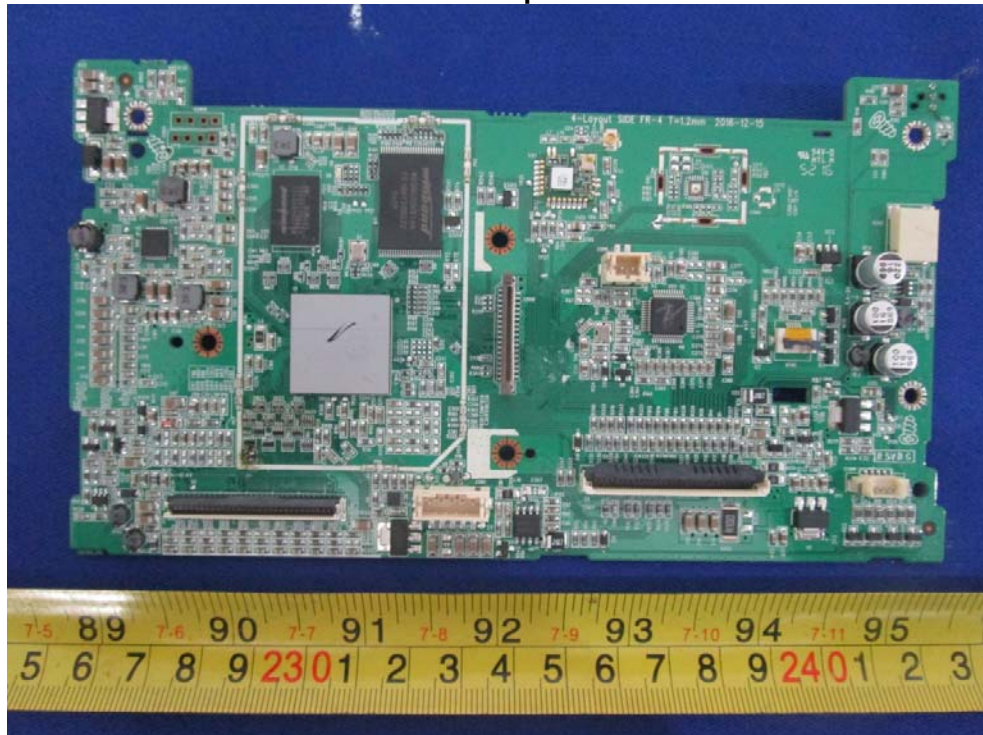
EUT – Subboard Top Uncover View
