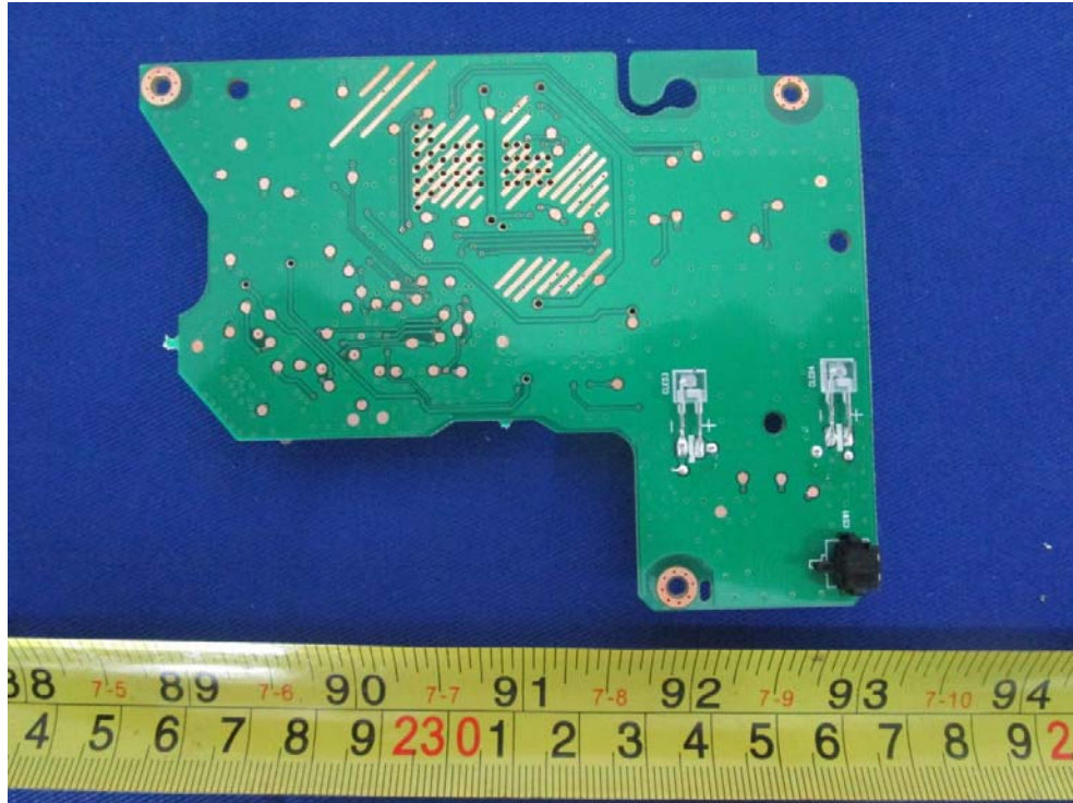
EUT – CD Board Bottom View
