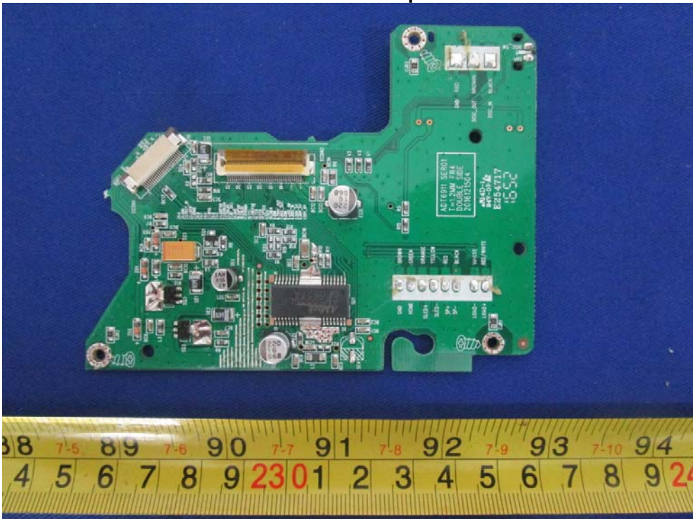
EUT – CD Board Top View
