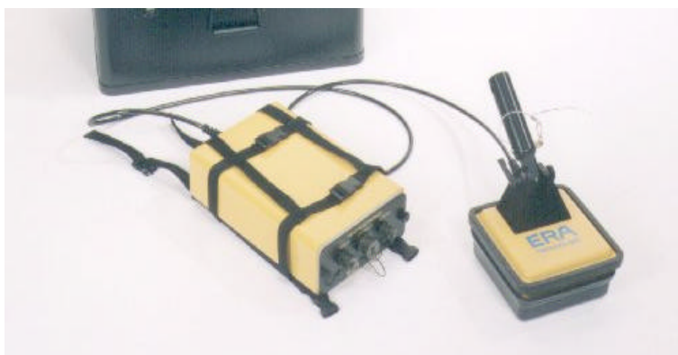
Figure 8 1GHZ antenna
