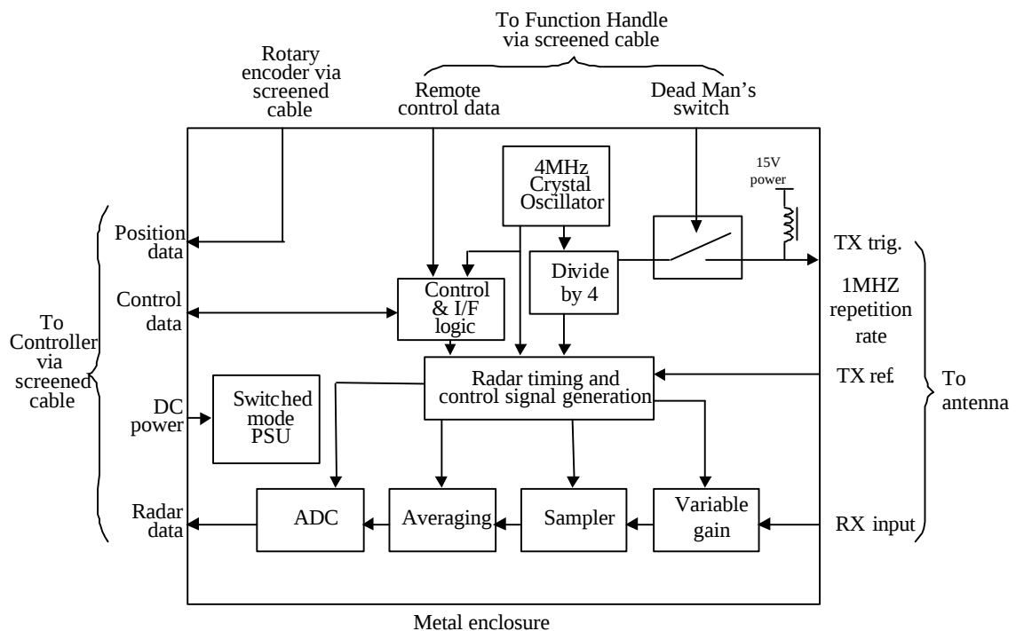
Fig. 7: SPRscan head electronics block diagram
