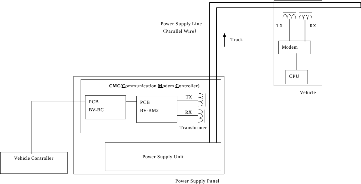
Fig. 1 Current CMC configuration (Already compliant to FCC Part 15 Subpart C)
