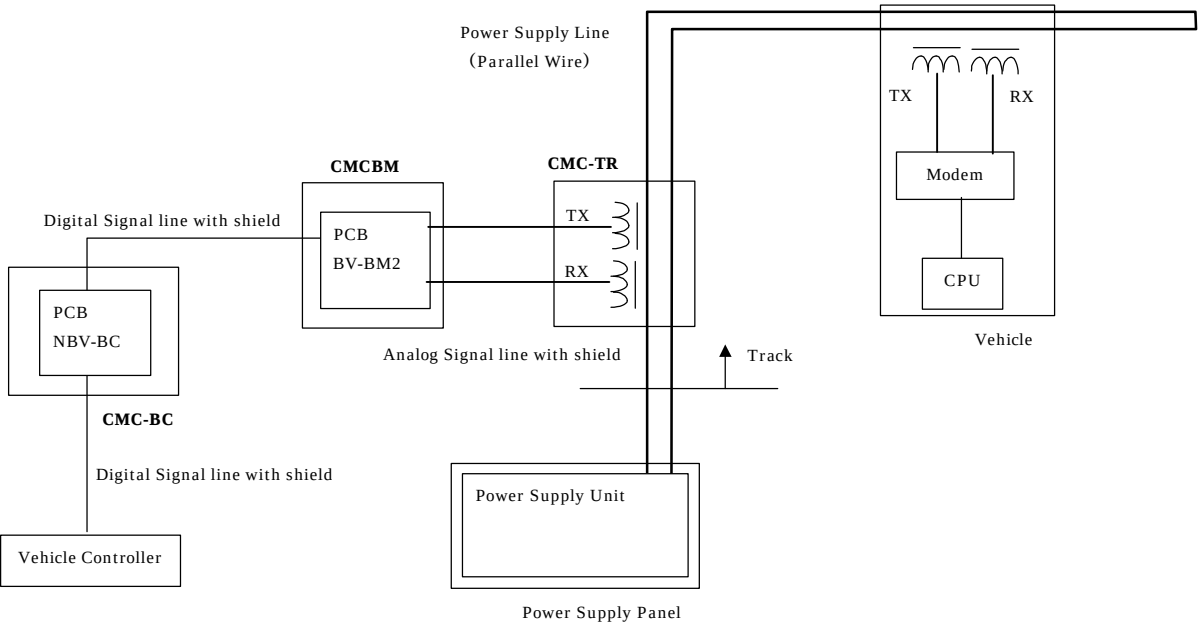
Fig. 2 Modified base CMC configuration
