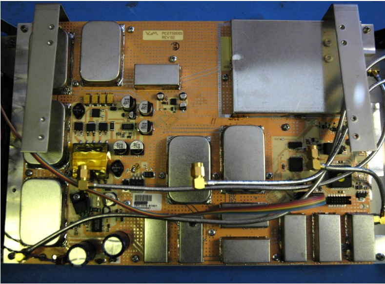
PCB – Shielded On View
