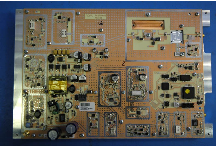
PCB – Shield off View
