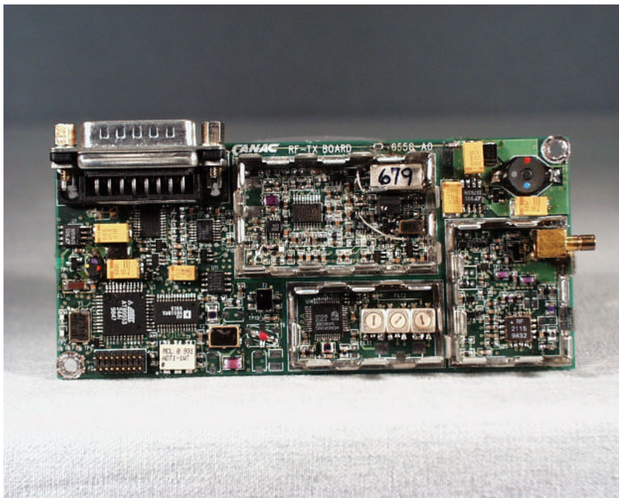
Component side of the board (with RF cans removed)
