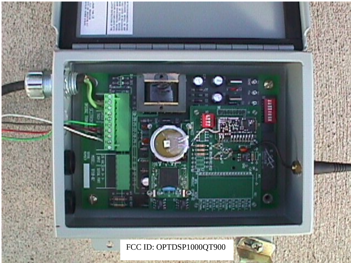
Internal View of Receiver
