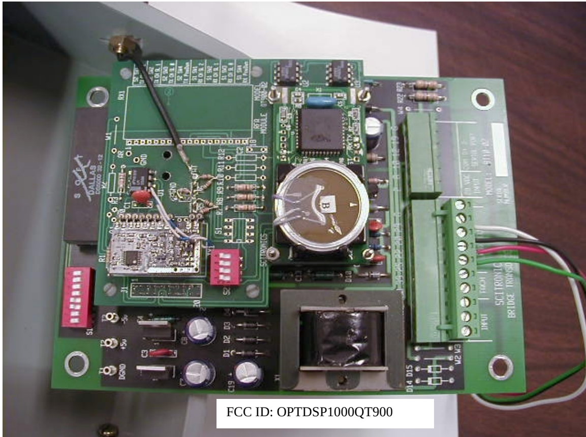
Front of Circuit Board for Receiver
