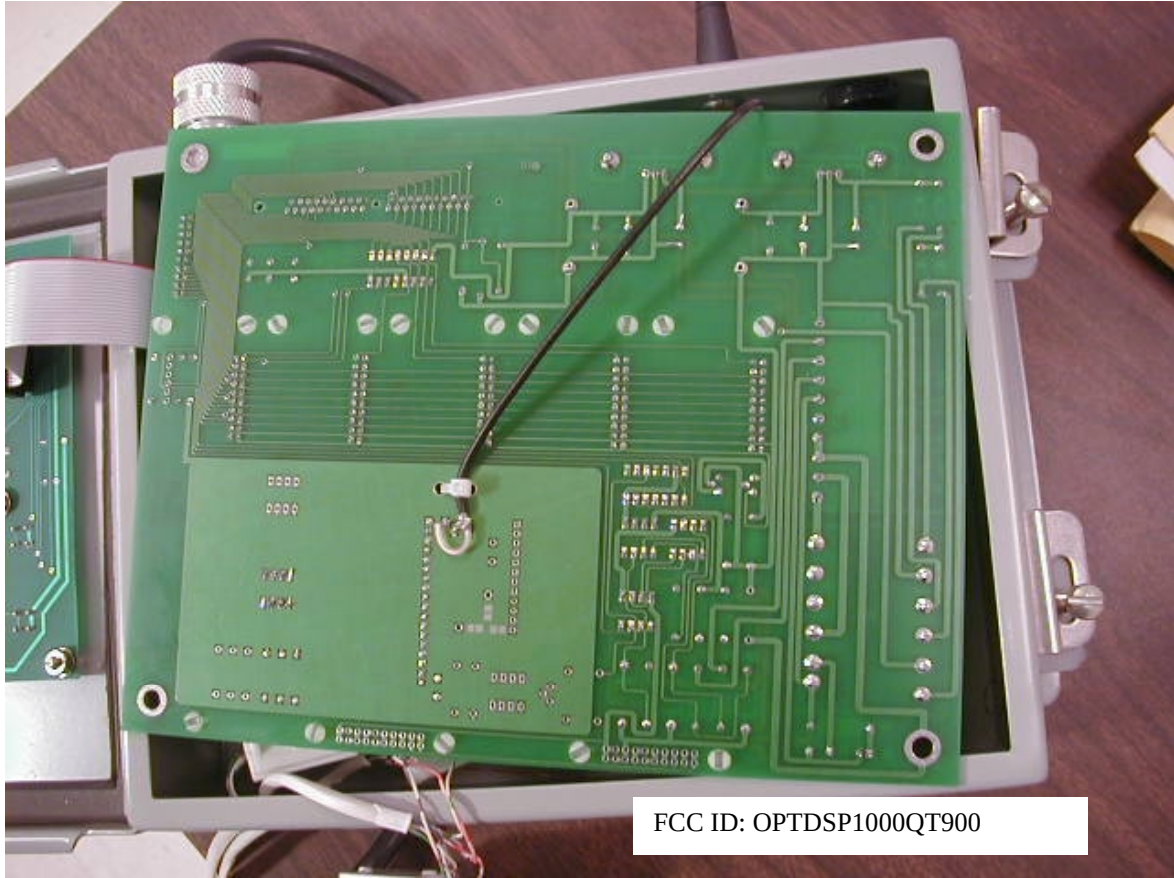
Back of Circuit Board for Transmitter
