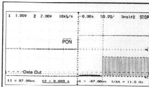
Figure 4: Receiver Turn-on Time
