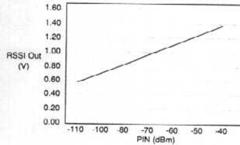
Figure 5: Receiver RSSI
