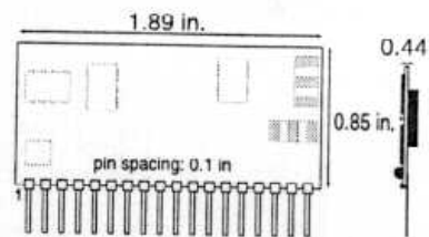
Figure 8: Physical package
