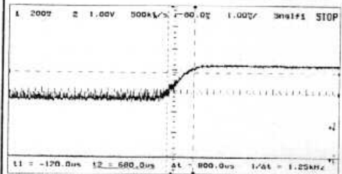
Figure 4: Receiver Turn-on Time
