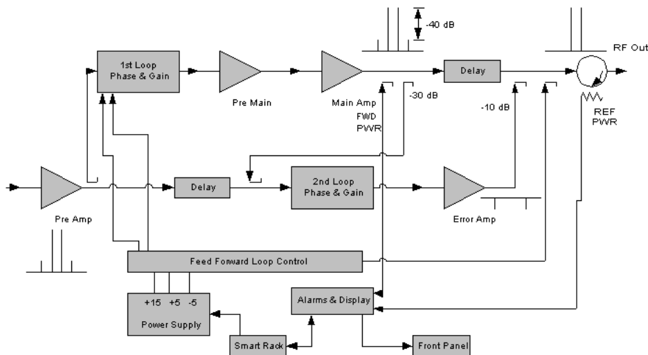
Multi-Carrier Power Amplifier Functional Block Diagram
