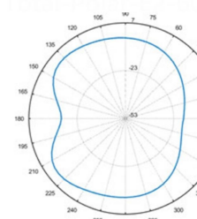
Total-Polar-E2-902MHZ
