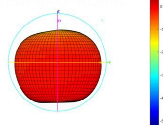
Total-3D-E2-930MHZ
