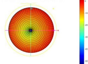
Total-3D-H-920MHZ
