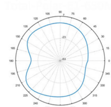
Total-Polar-E1-920MHZ
