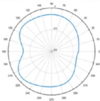
Total-Polar-E1-930MHZ
