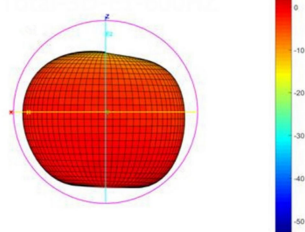
Total-3D-E1-902MHZ
