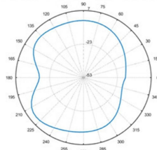
Total-Polar-E1-902MHZ
