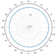
Total-3D-H-930MHZ
