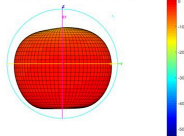
Total-3D-E2-902MHZ
