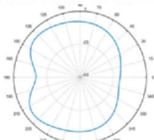
Total-Polar-E2-920MHZ
