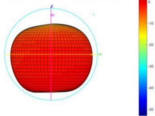
Total-3D-E2-920MHZ
