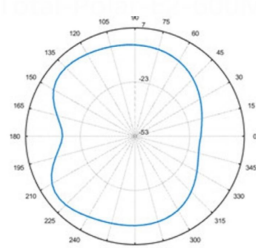
Total-Polar-E2-902MHZ
