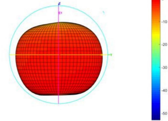
Total-3D-E2-930MHZ
