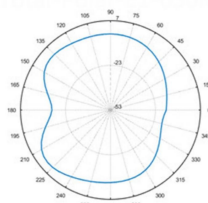
Total-Polar-E1-920MHZ
