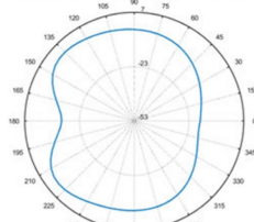
Total-Polar-E2-930MHZ
