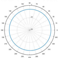
Total-3D-H-930MHZ
