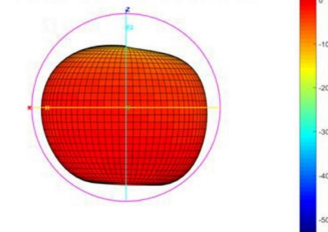
Total-3D-E1-920MHZ
