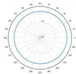
Total-Polar-H-902MHZ
