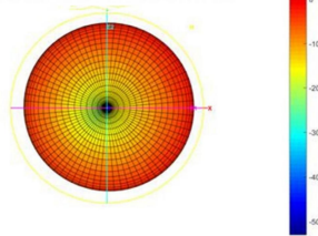
Total-3D-H-920MHZ
