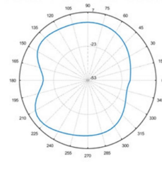
Total-Polar-E1-902MHZ
