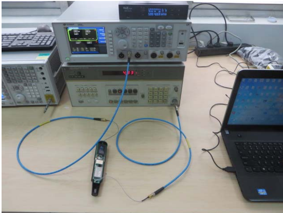
Conducted Test 2
