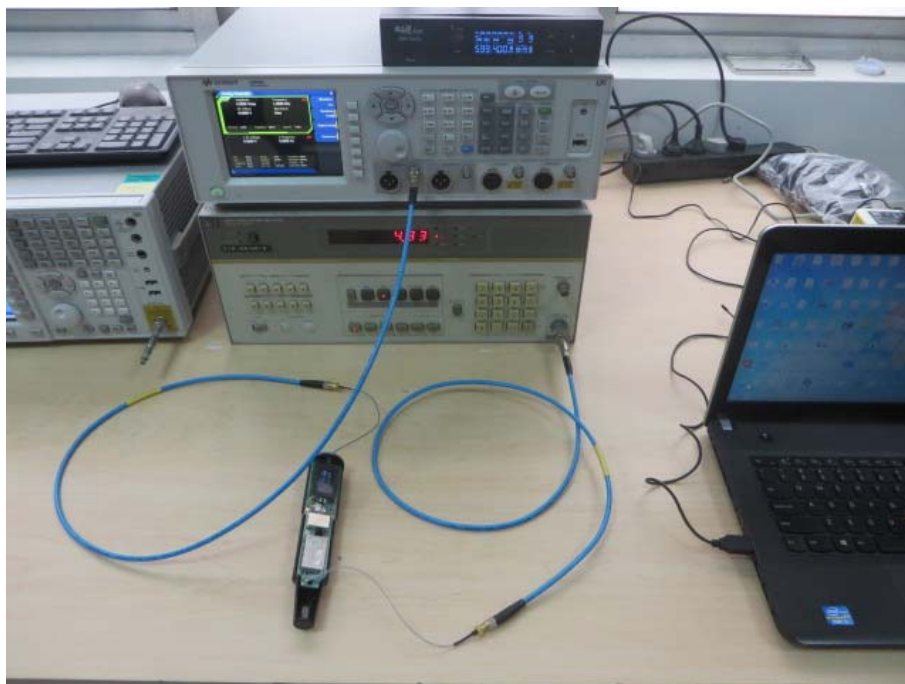
Conducted Test 2
