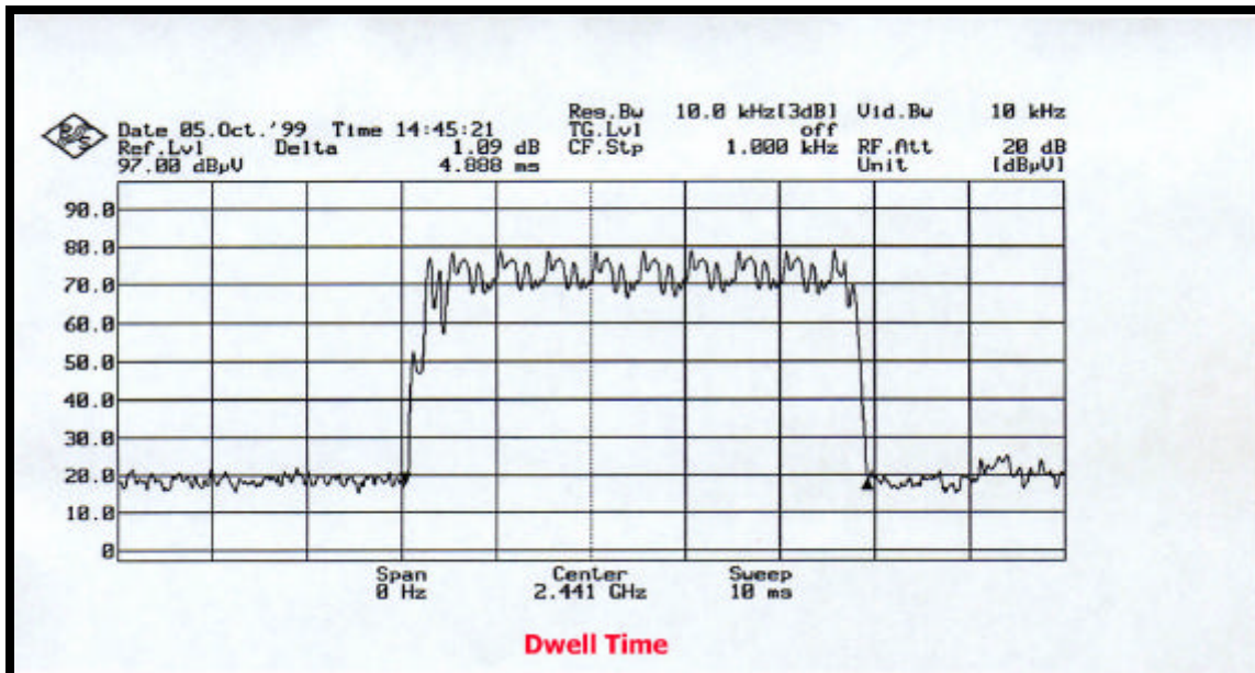
Test Data : Plot – Dwell Time – Port 1
