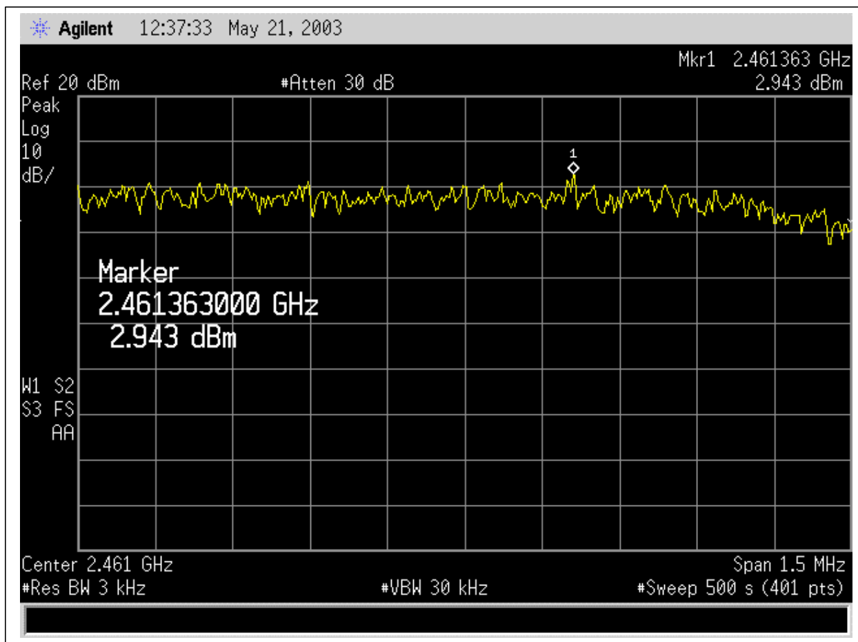
Graph # 3-5-6 Peak Power Spectral Density, Channel 11, No Amplifier Limits: 7.65dBm
