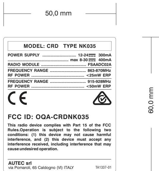
CRD label and its dimension
