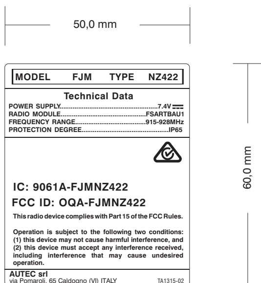
FJM label and its dimension
