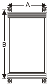
Drilling template A=106 mm B=213,5 mm
