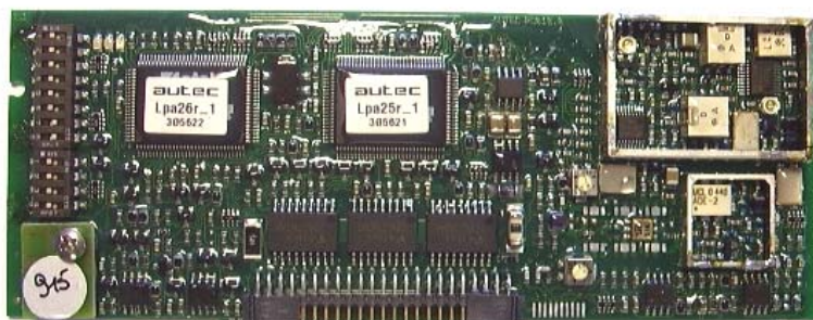
Radio Module without shield
