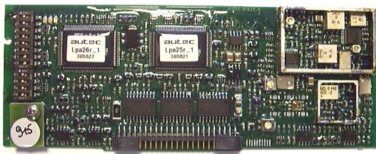
Radio Module without shield
