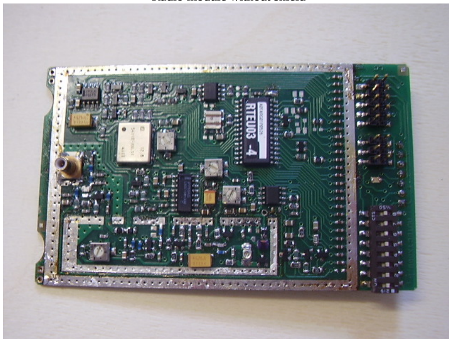
Radio module without shield
