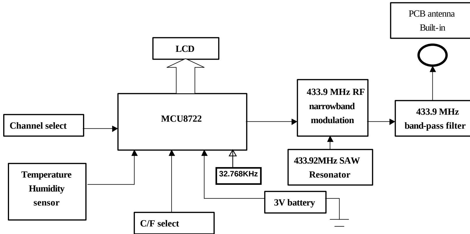
Figure 1 C8202FCC Block diagram
