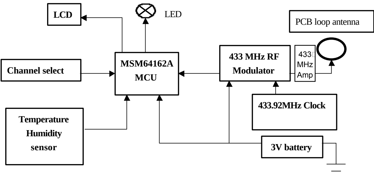
Figure 2 C8102 Block diagram
