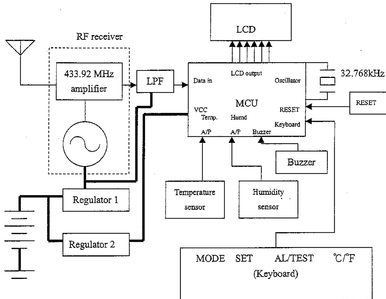
C810/ C813 block diagram
