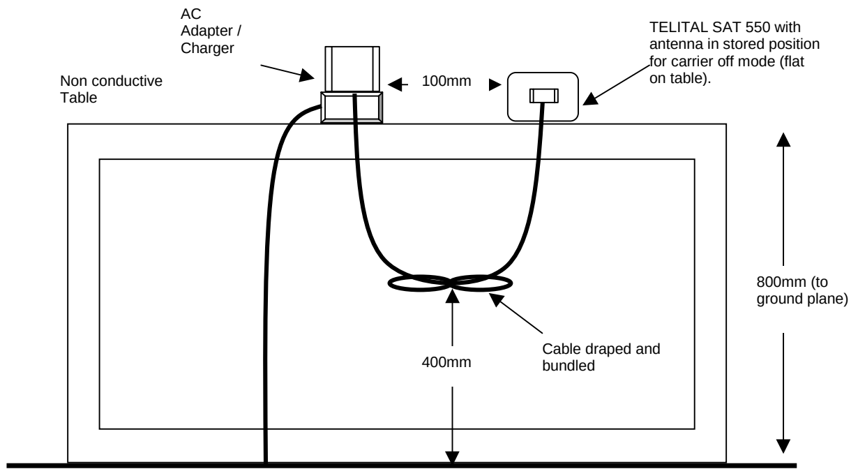
Figure 2: Telital SAT 550 CFR 47 Part 15.109 Radiated Emission Set up (Rear View)
