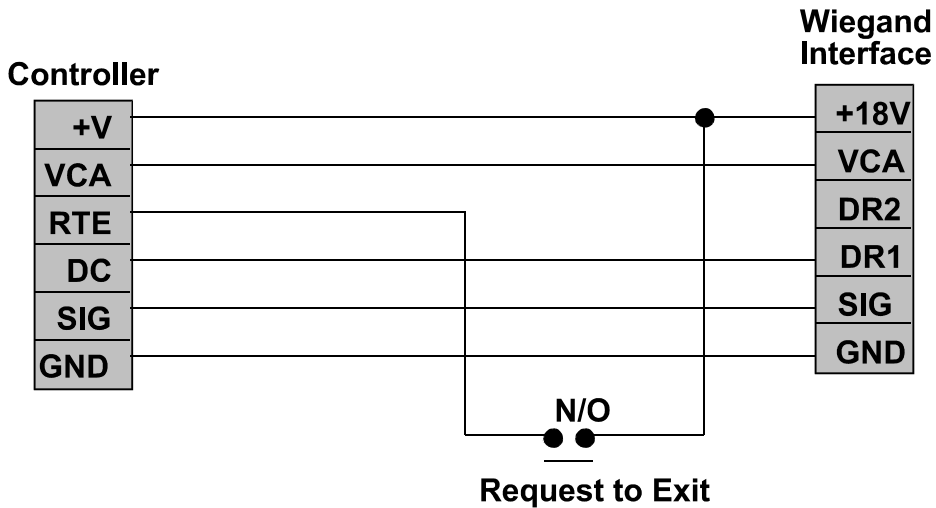
Figure 8 Easikey 1000 Controller to Wiegand Interface Wiring Diagram
