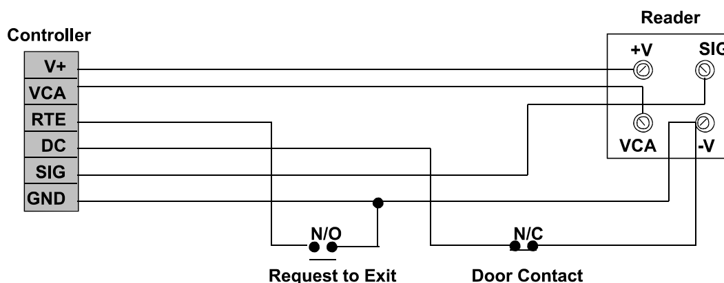
Figure 5 Proximity Reader Wiring Diagram
