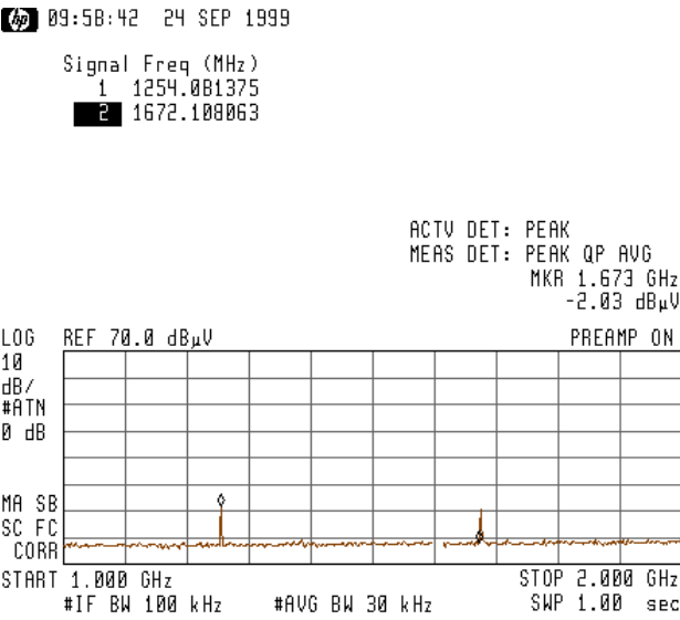
Plot of frequencies from 1 to 2 GHZ
