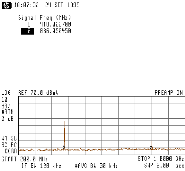
Plot of frequencies from 200 to 1000 MHZ
