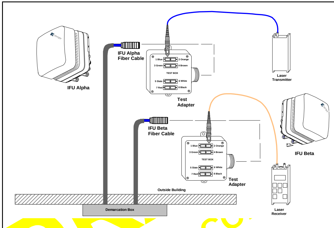
Figure 3-11. Fast Ethernet Fiber Optic Continuity Test Setup
