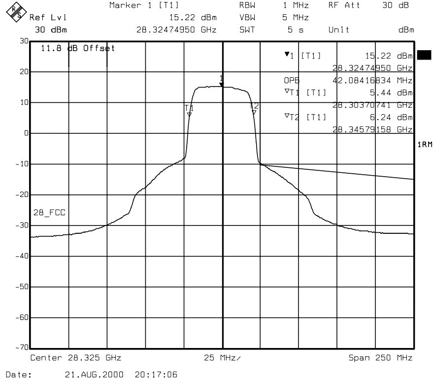
Figure 5. – 32 QAM, 1Watt output at the high end of the band – Actual power 29.57dBm
