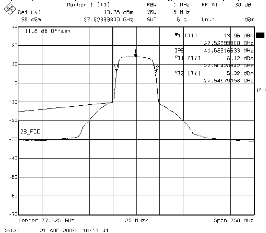
Figure 2. – 32 QAM , 1Watt output at the lower band edge. Actual output power 28.33 dBm
