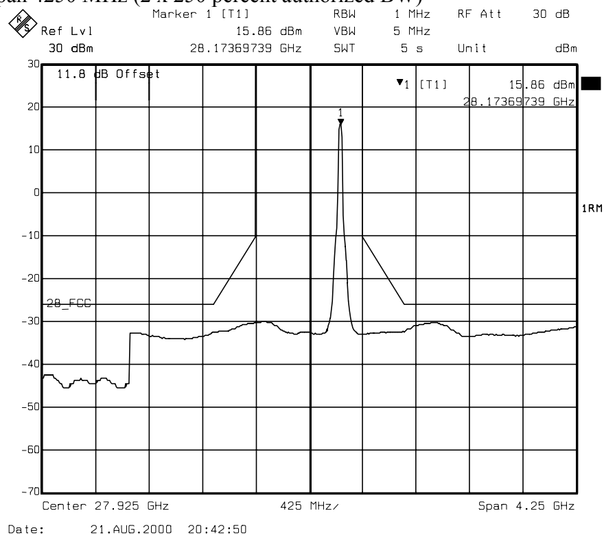
Figure 6. – span 4250 MHz (2 x 250 percent authorized BW)
