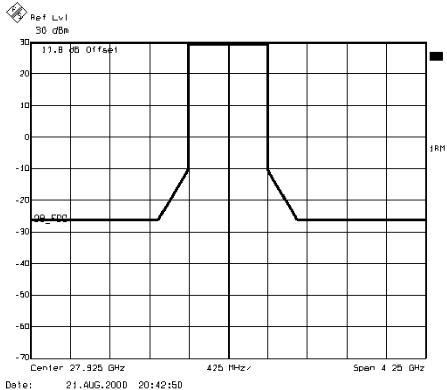
Figure 1. FCC mask for the 28 GHz band
