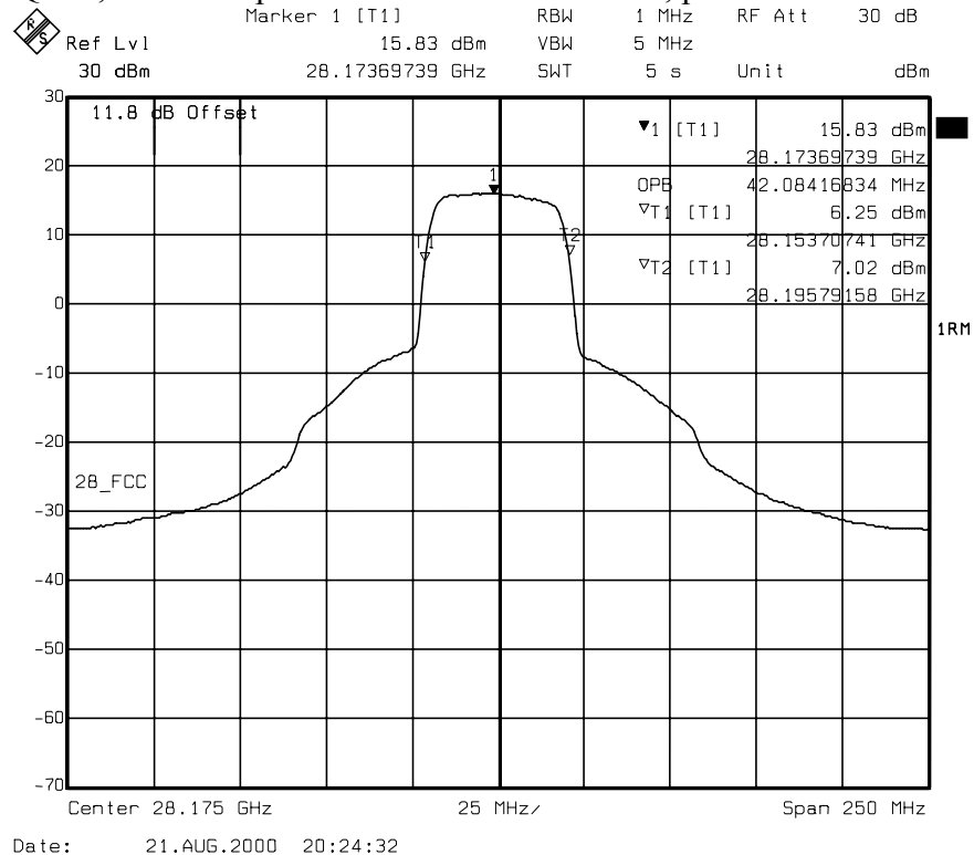
Figure 4. – 32 QAM, 1Watt output in the middle of the band, power 29.89dBm
