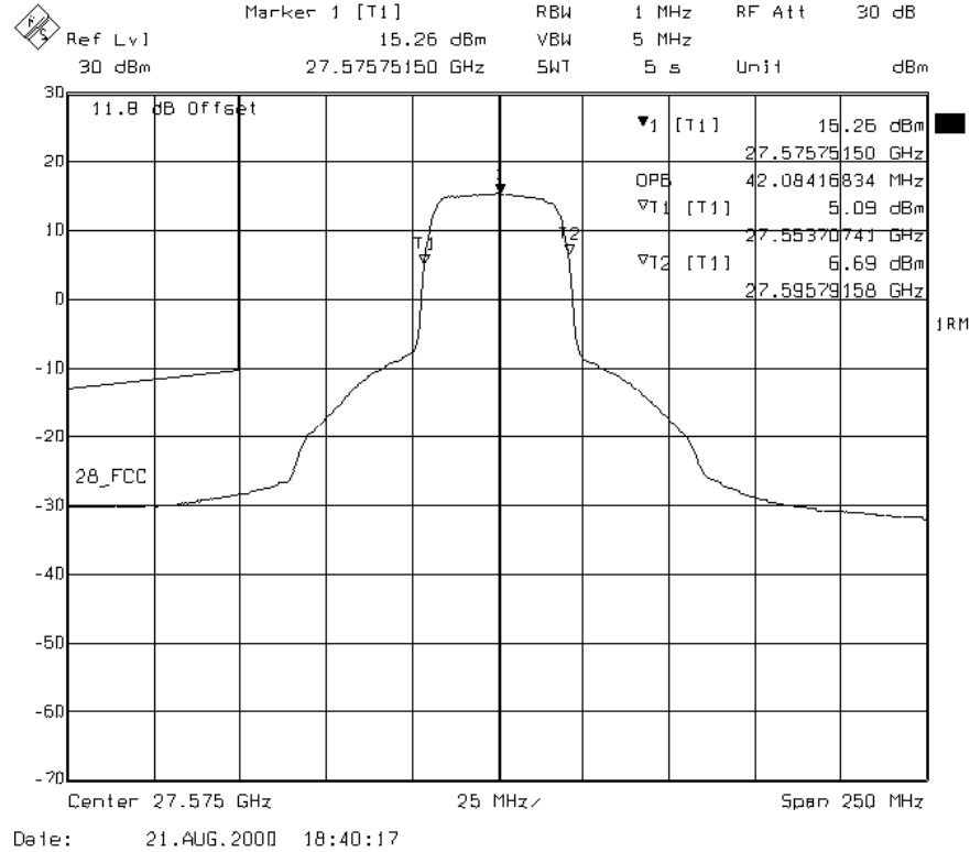
Figure 3. – 32 QAM, 1Watt at the lower band edge – next channel - actual power 29.33dBm
