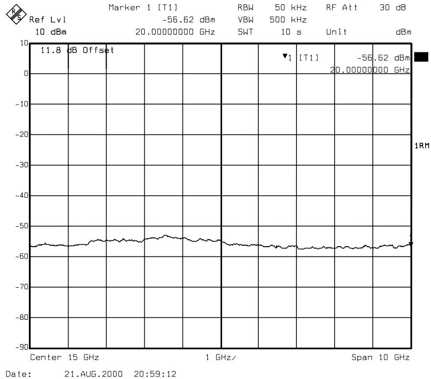
Figure 8. Spurious emissions at low output power: -4dBm
