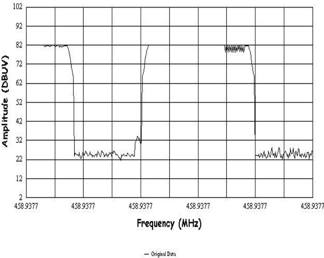
FIGURE 1: MODULATION CHARACTERISTICS PLOT
