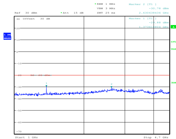
Figure 8.4-20: Conducted spurious emissions above 1 GHz for SOQPSK modulation, high channel
