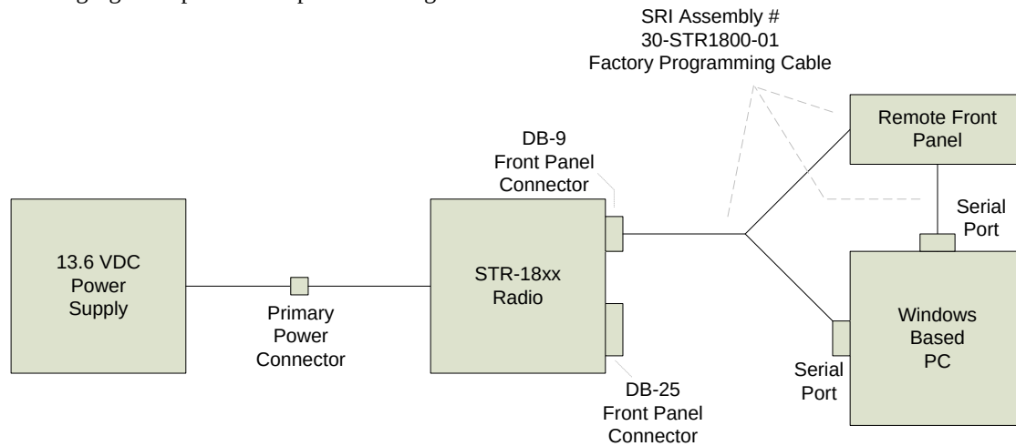
Figure 5 Factory Radio to PC Interconnect Configuration
