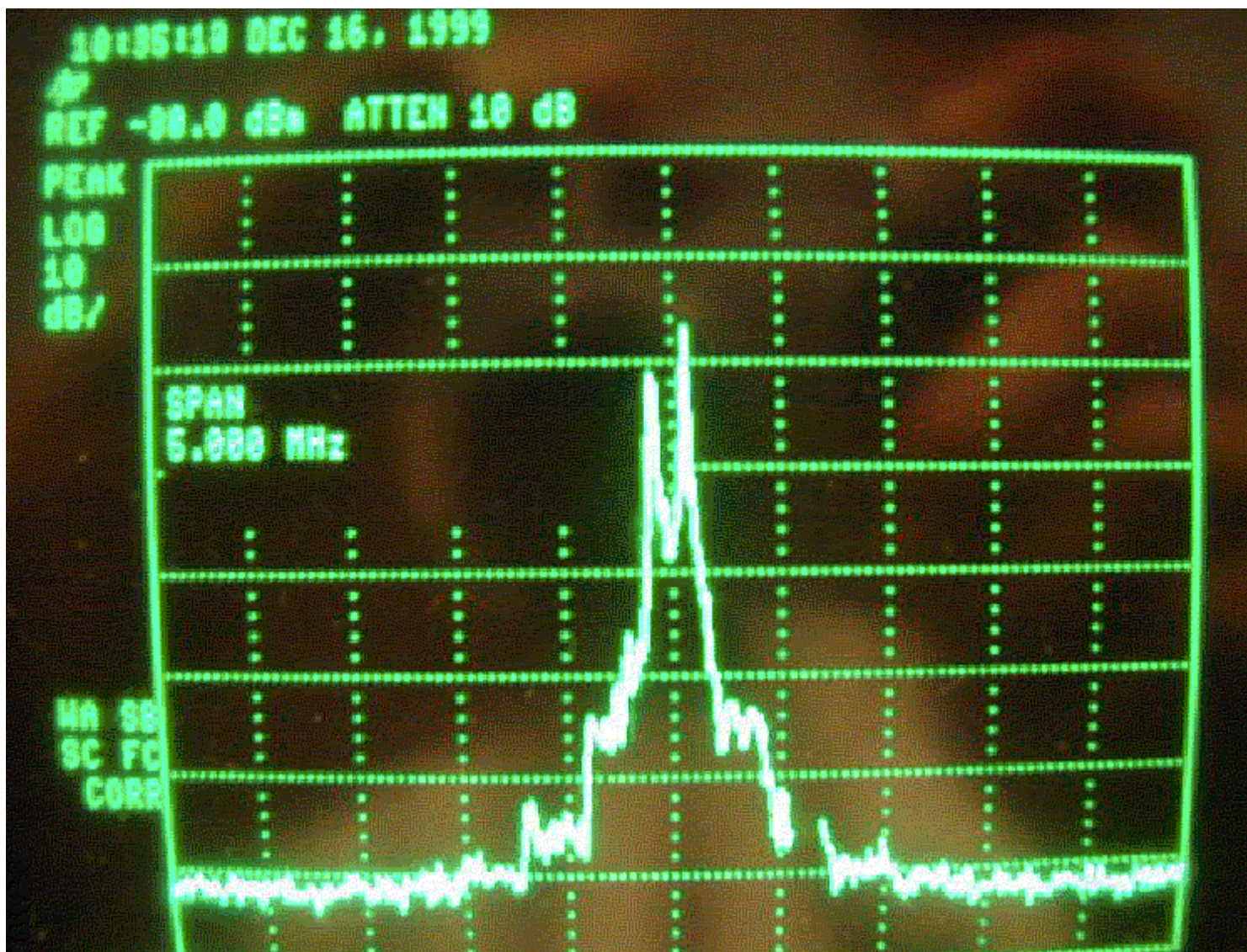
Bandwidth Spectrum Picture of ST-326 Transmitter Operating at 923.37 MHz
