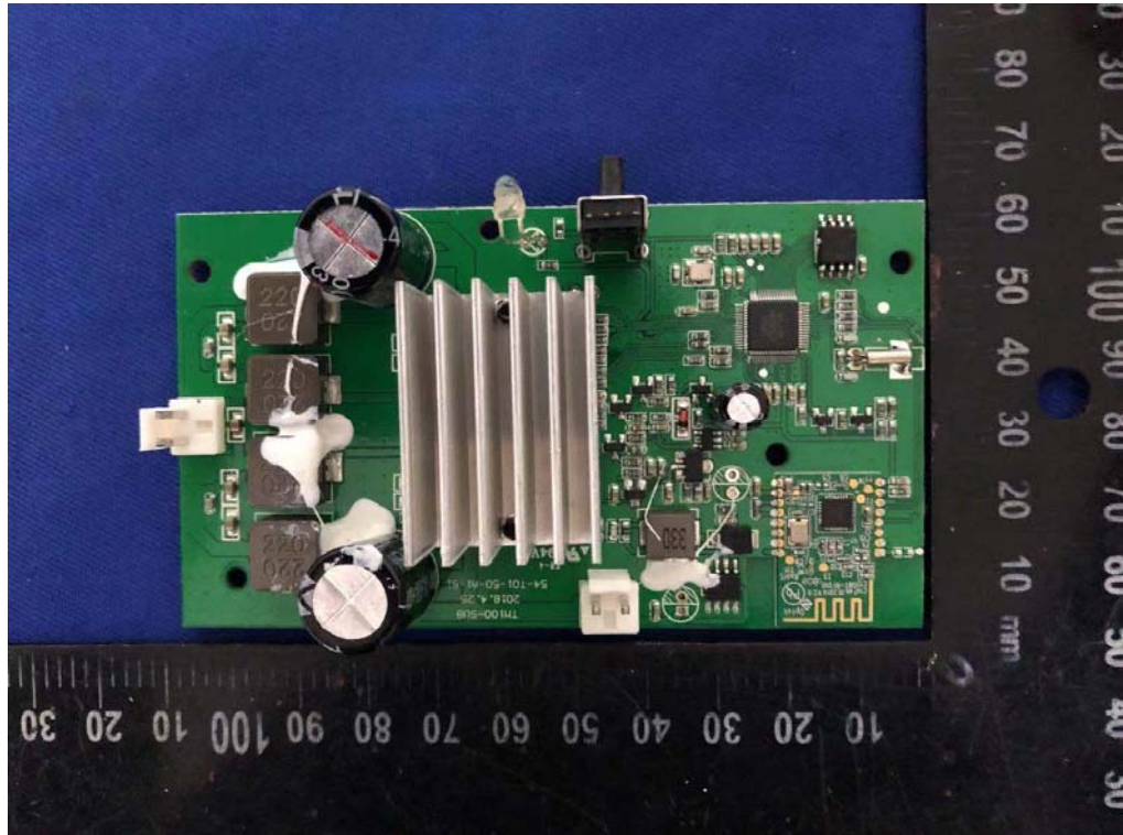
Internal Photos M/N: R-4B II NA Subwoofer
