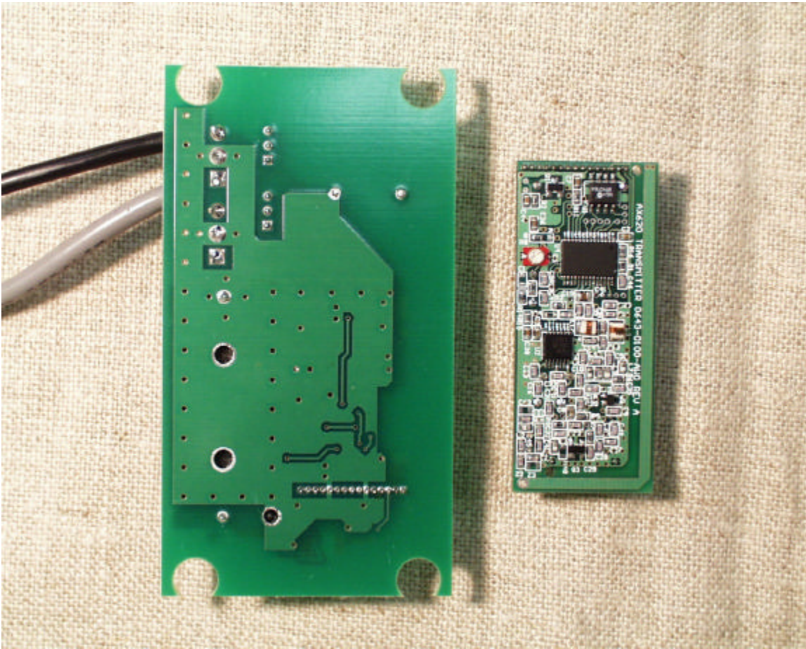
PCB Bottom with AX-620 transmitter removed
