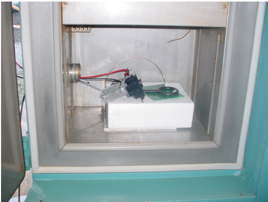
Frequency Stability
