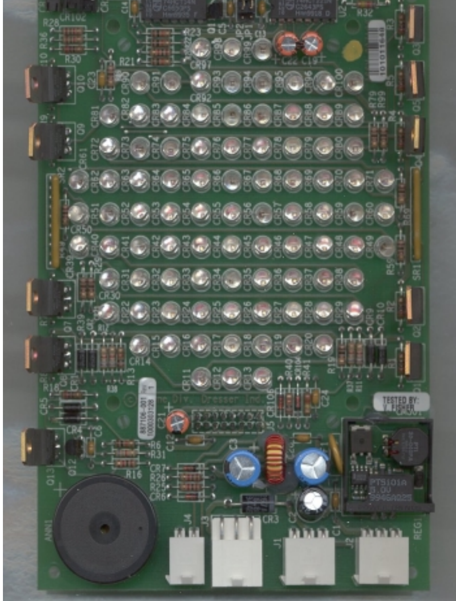
Assembly, Lite Board, Shell, Component Side
