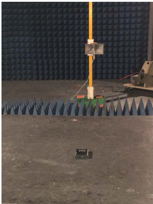
Radiated emissions test > 1GHz
