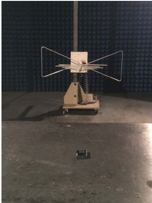
Radiated emissions test 30MHz- 1GHz
